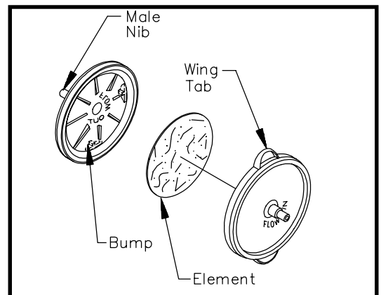
Figure 25. VisiFilter Element Replacement
