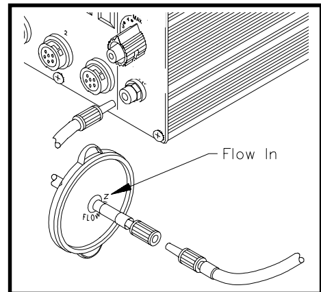
Figure 10. VisiFilter Preparation
