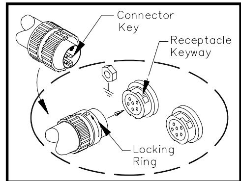
Figure 5. Handpiece Connection
