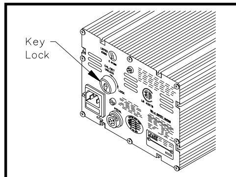
Figure 14. Key Lock
